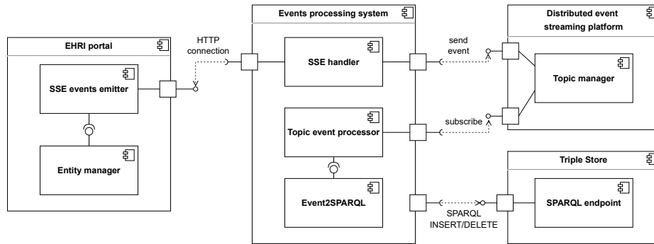
Fig. 2. Architecture of the envisioned stream-based incremental update system to align the KB with the EHRI Portal’s live dataset where the EHRI portal will emit events in the form of Server-Sent Events (SSE). A SSE handler will process and send them to a topic in a distributed event streaming platform (e.g., Apache Kafka). Finally, an event processor will be subscribed to the event streaming platform and will create (and post to the SPARQL endpoint of the triple store) the corresponding SPARQL INSERT and/or DELETE queries based on the events contents.
