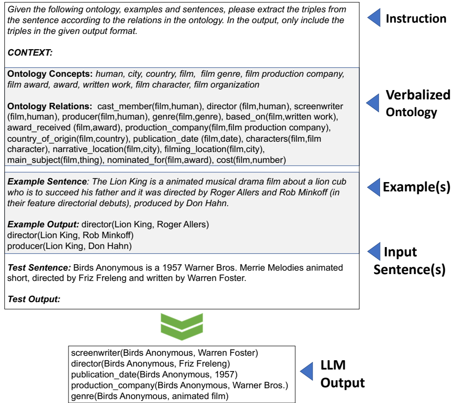
Fig. 2. An example prompt for an instruction fine-tuned LLM and the generated output from the LLM model.
