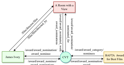
Fig. 1: A small fragment of Freebase, with a mediator node
