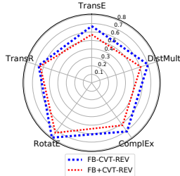
Fig. 3: Impact of mediator nodes on MRR^\uparrow of embedding models
