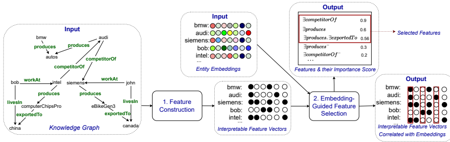
Fig. 1: Embedding-guided feature vector generation for KG entities
